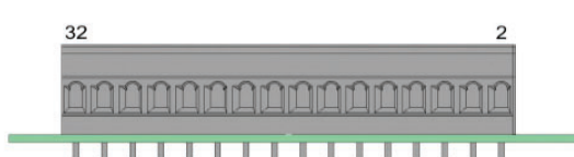
Spring clamp terminals (Max. 12A / terminal)
